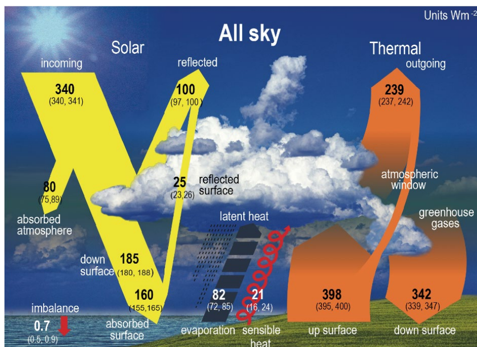
Figure 15. The global mean energy budget of Earth according to IPCC AR6 [2] (Section 7.2.1), their Figure 7.2. Numbers indicate the best estimates for magnitudes of the globally averaged energy balance components in \text{W m}^{-2} , together with their uncertainty ranges in parentheses (5–95% confidence range), representing all-sky climate conditions at the beginning of the 21st century. According to this diagram, the Tropospheric Energy-Flux Attenuation Coefficient (TEFAC) is 239/(398 + 82 + 21) = 0.477 .
